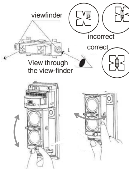
Fig. 5 Setting up the optical part
